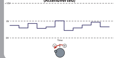
Figure 28: Random Stepped Voltage (Attenuverted)
