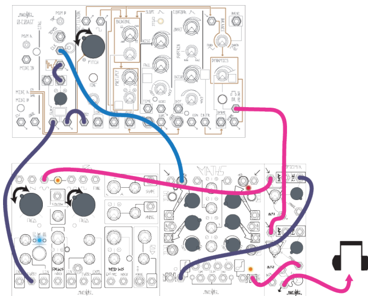
Figure: 69 Any CV or Gate signal conforming to these signal levels may be used to control the 0-Coast, and vice versa.
