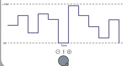
Figure 25: Random Stepped Voltage
